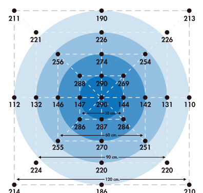
SLIMSUNPRO240W@90cm PPFD = 290
